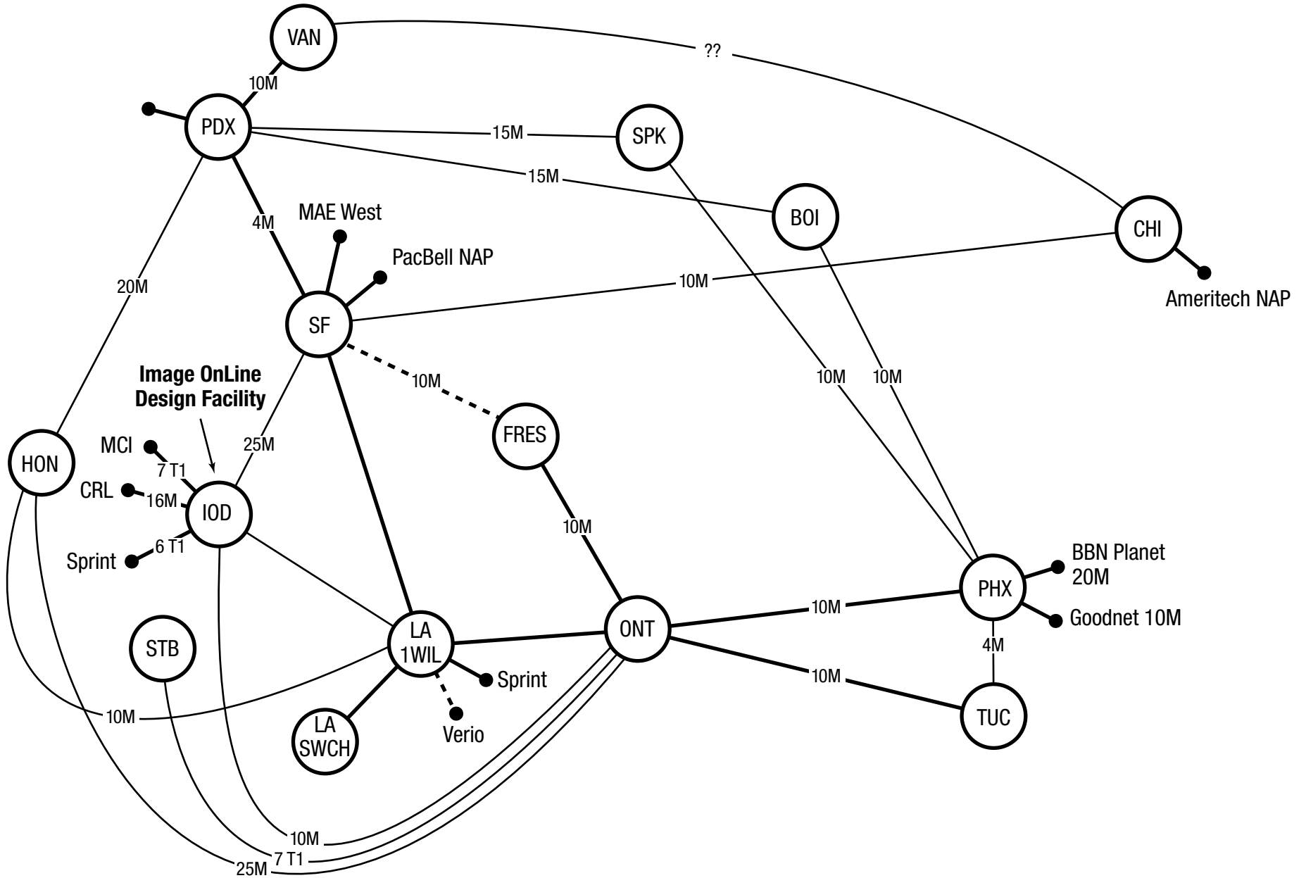
Fig. D15.2.1_E INTERNET CONNECTION TOPOLOGY
