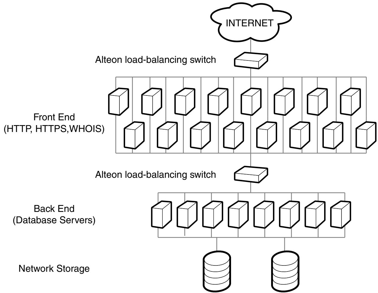
Fig. D15.2.1_C NETWORK TOPOLOGY
